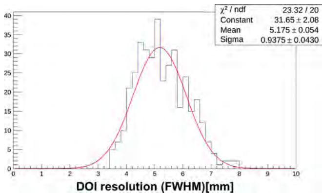
Fig. 8. Distribution of the DOI resolution for all the 64 crystals.
