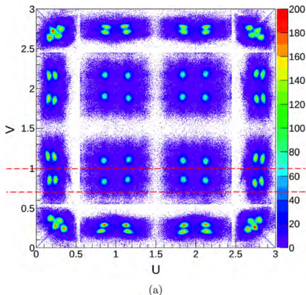
Fig. 4. (a) Corrected flood histogram and (b) the corresponding projection for the selected crystals.
