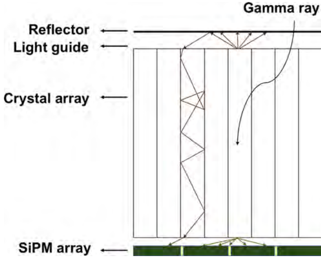
Fig. 1. Schematic representation of the DOI encoding method.
