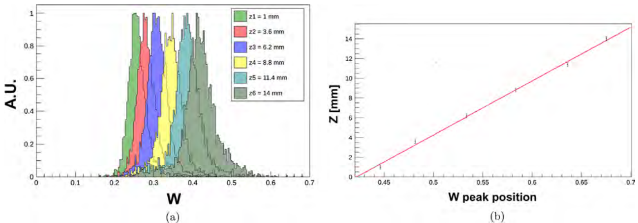
Fig. 7. (a) Histograms of the W variables for 6 different z positions along the crystal length for 511 keV events in photopeak and (b) the linear correlation between the centers of the irradiation spots and the positions of the W histogram peaks.
