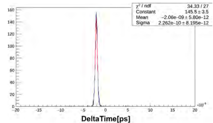
Fig. 9. Distribution of time difference between two modules in coincidence.
