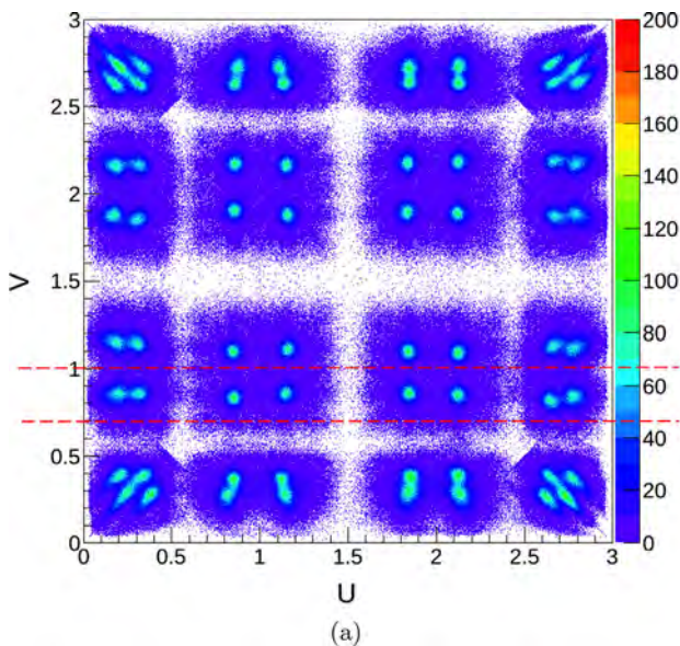
Fig. 2. (a) Flood histogram and (b) the corresponding projection for the selected crystals.
