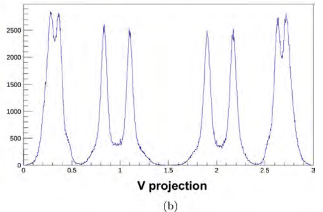
Fig. 2. (a) Flood histogram and (b) the corresponding projection for the selected crystals.
