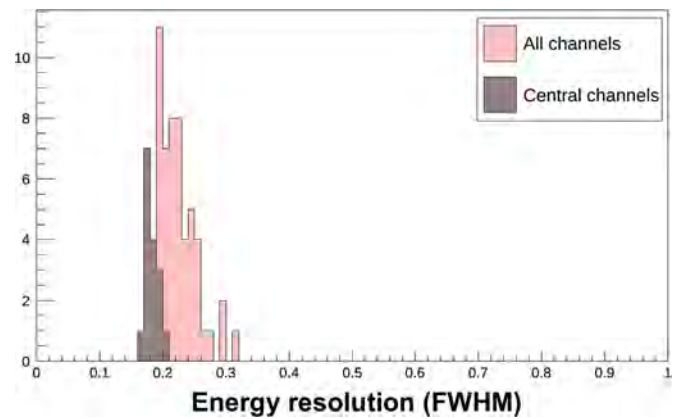
Fig. 5. Distribution of 511 KeV FWHM energy resolution.
