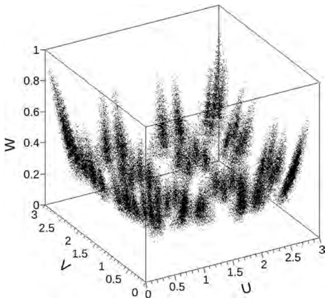
Fig. 3. 3D flood histogram of the variables (U, V, W) .
